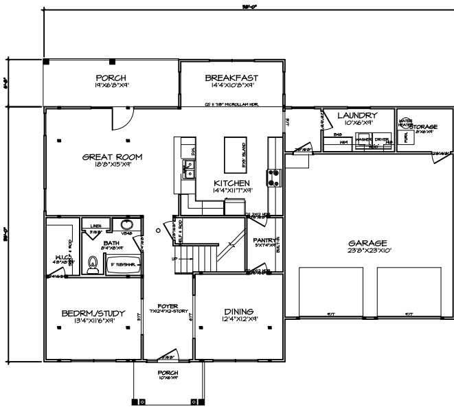
FIRST FLOOR PLAN A-4
