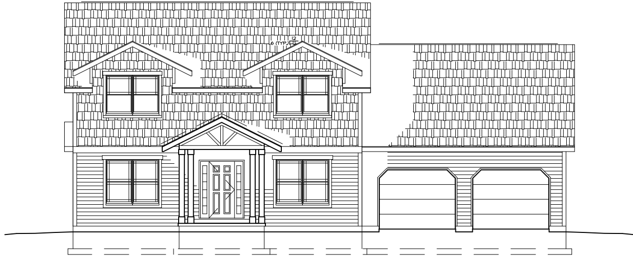
SOUTH ELEVATION A-1
