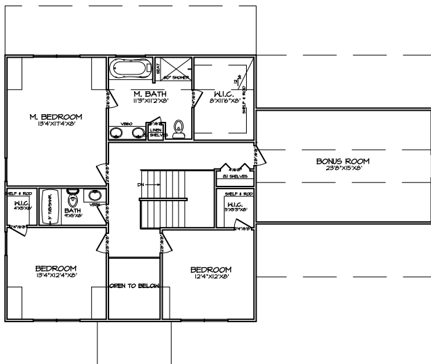
SECOND FLOOR PLAN A-5
